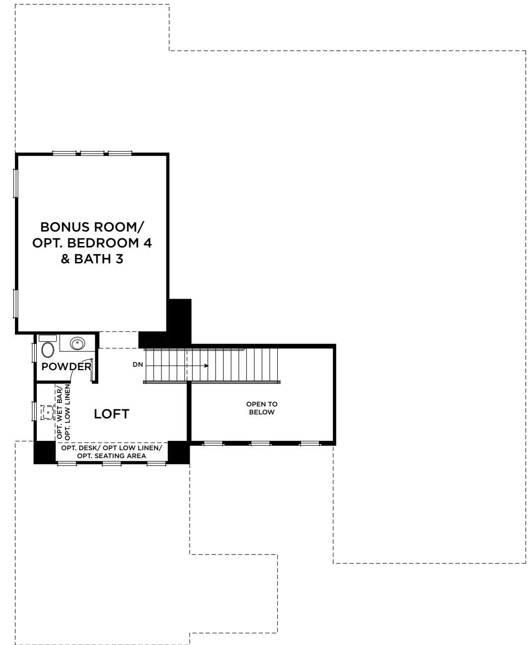
Optional 2nd Floor Plan
