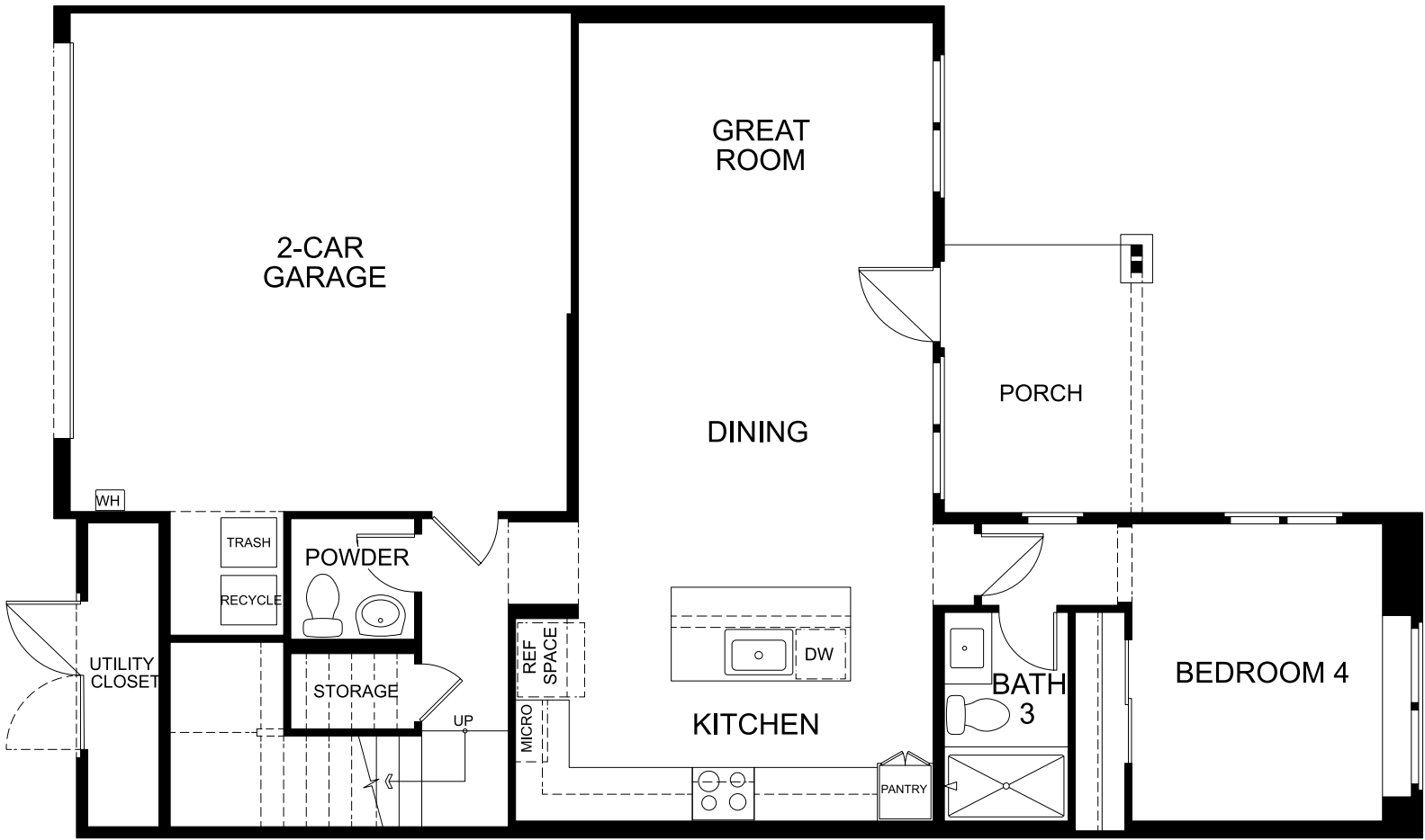
FIRST FLOOR
